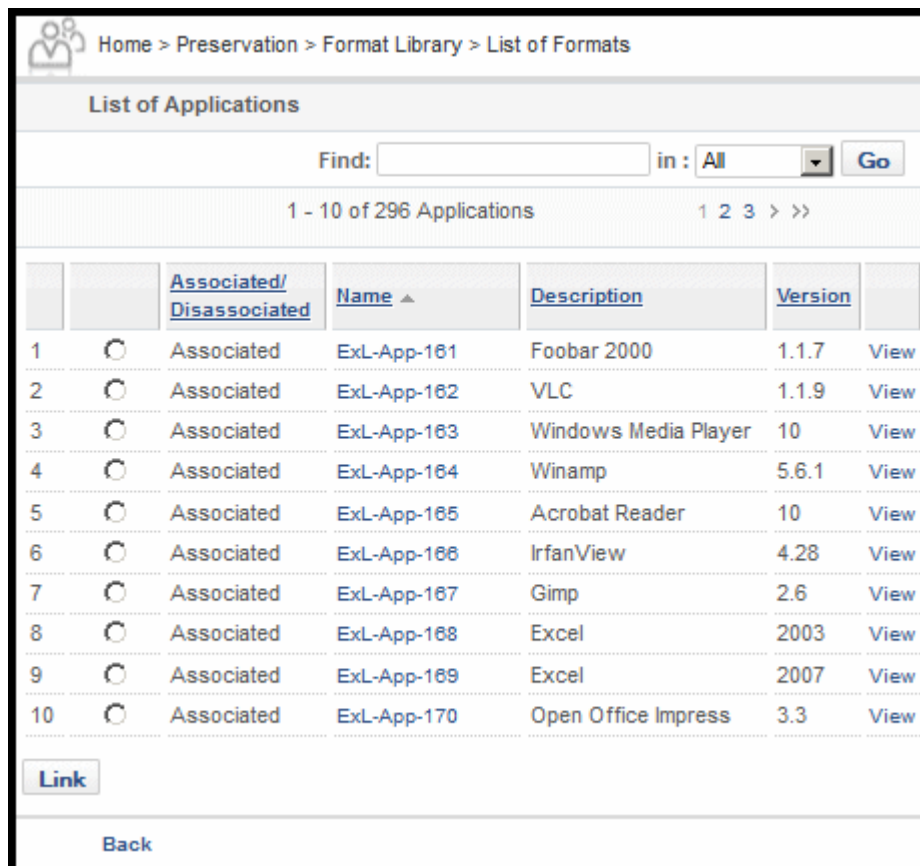
Figure 24: Associating Applications
