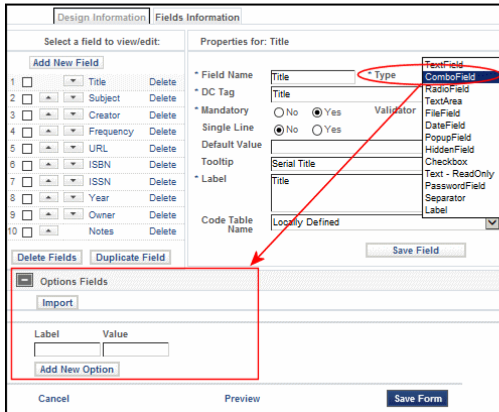
Figure 29: Metadata Form for New ComboField
