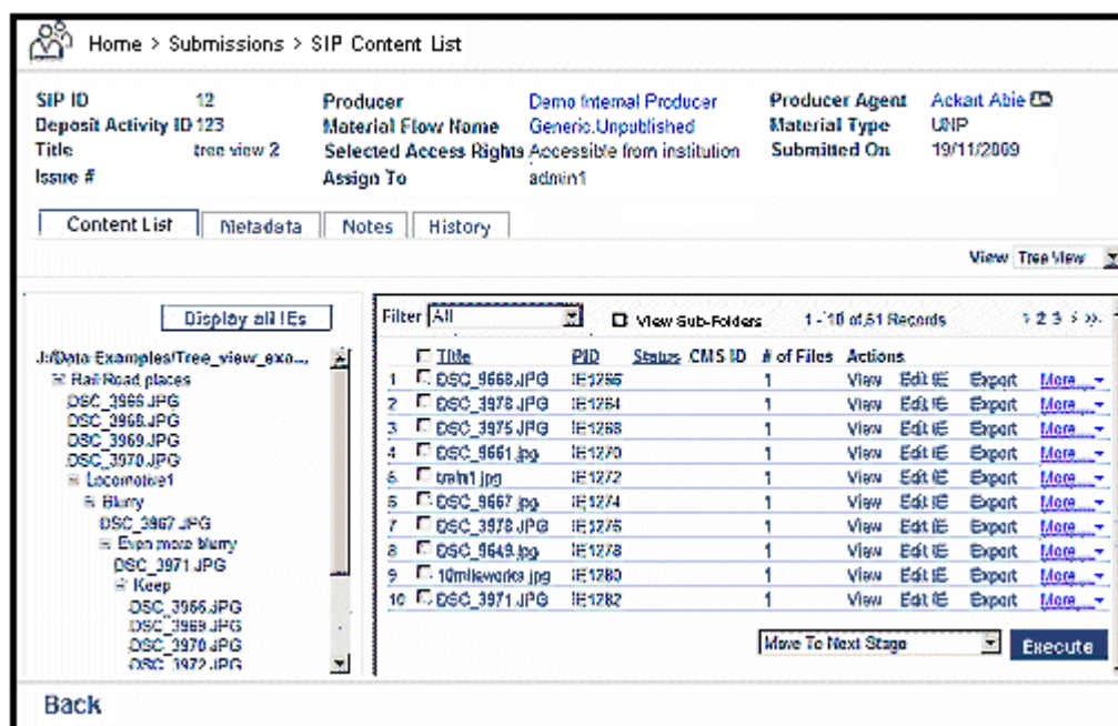
Figure 150: Tree View, Filters and Sub-folder View Options
