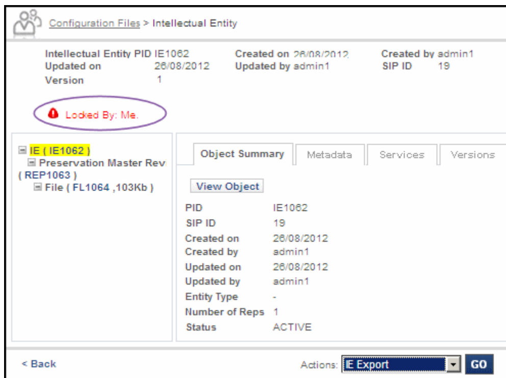
Figure 292: IE Locked by the User
