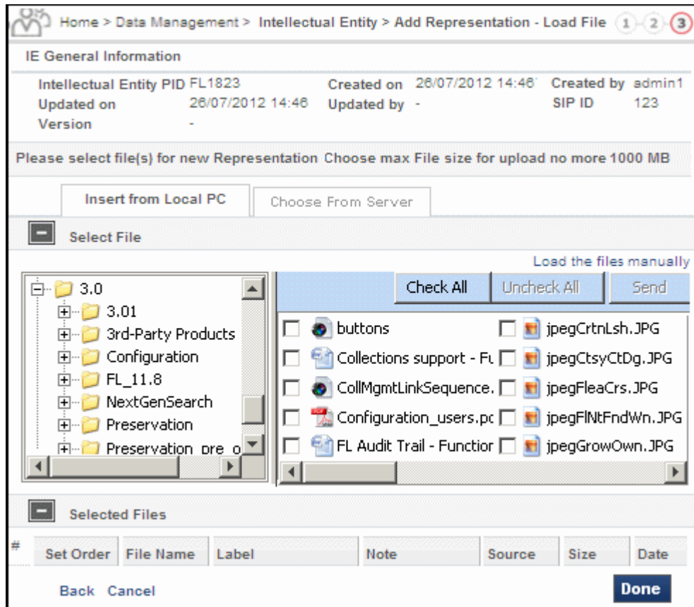
Figure 295: Add Representation - Load File
