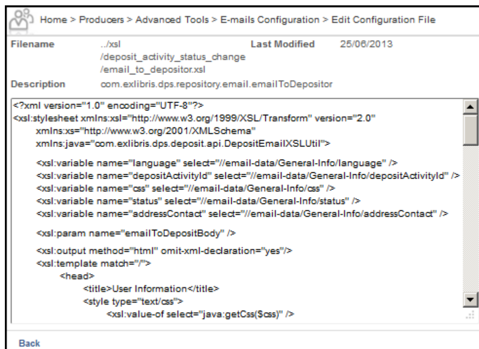
Figure 54: Editing a Configuration File
