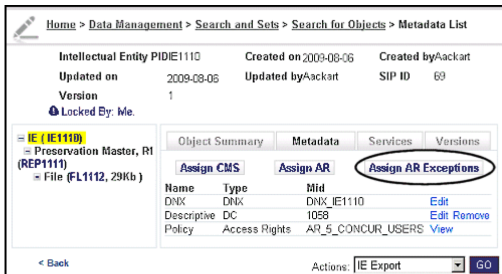
Figure 77: Assigning AR Exceptions to IEs
