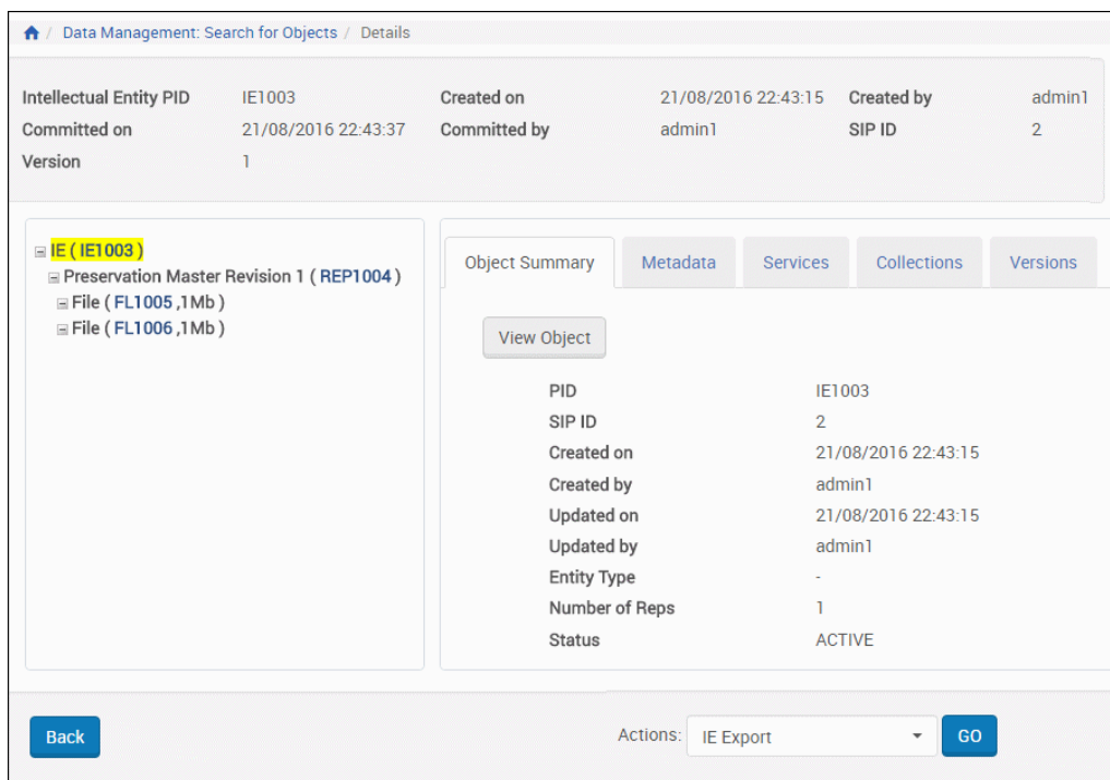
Figure 257: Web Editor Displaying IE Information
