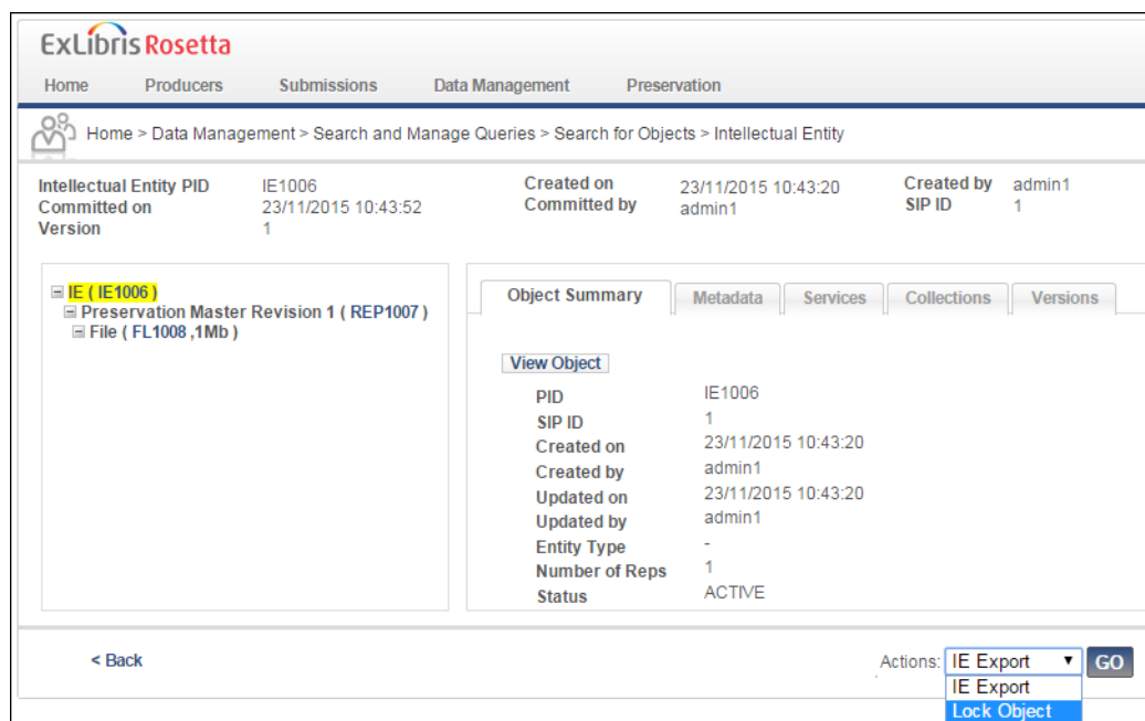
Figure 296: Open and Lock Object
