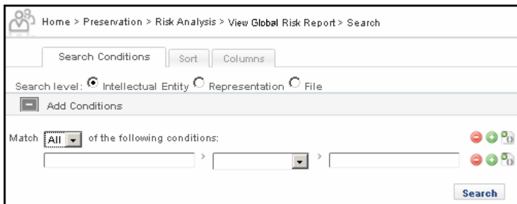
Figure 95: Search Page
