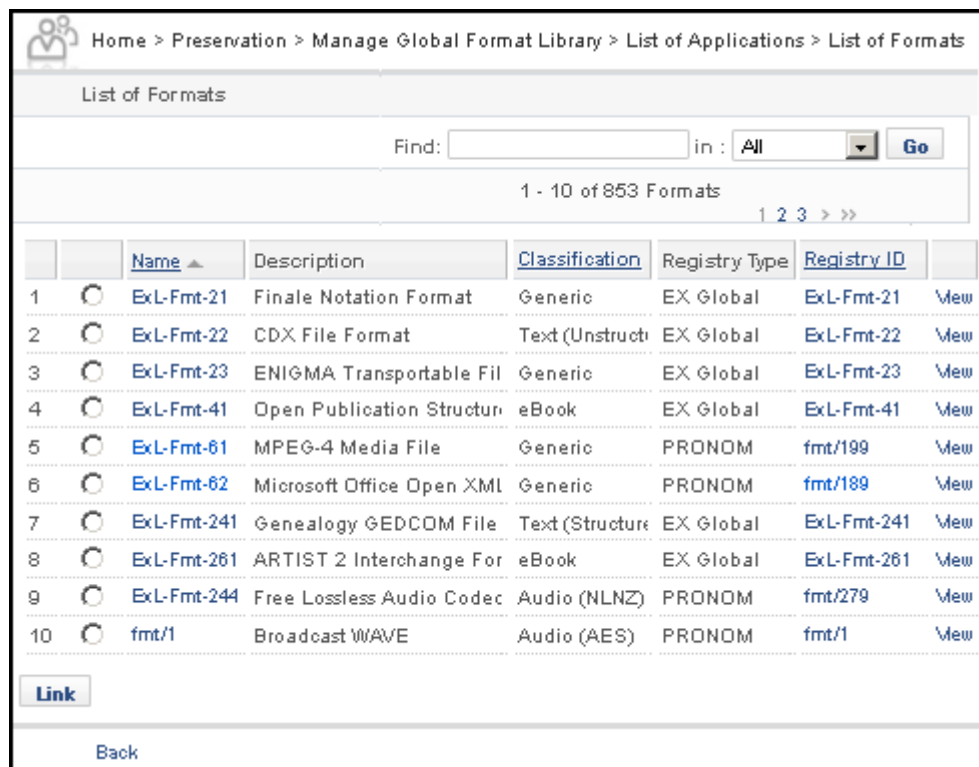
Figure 40: Add Format
