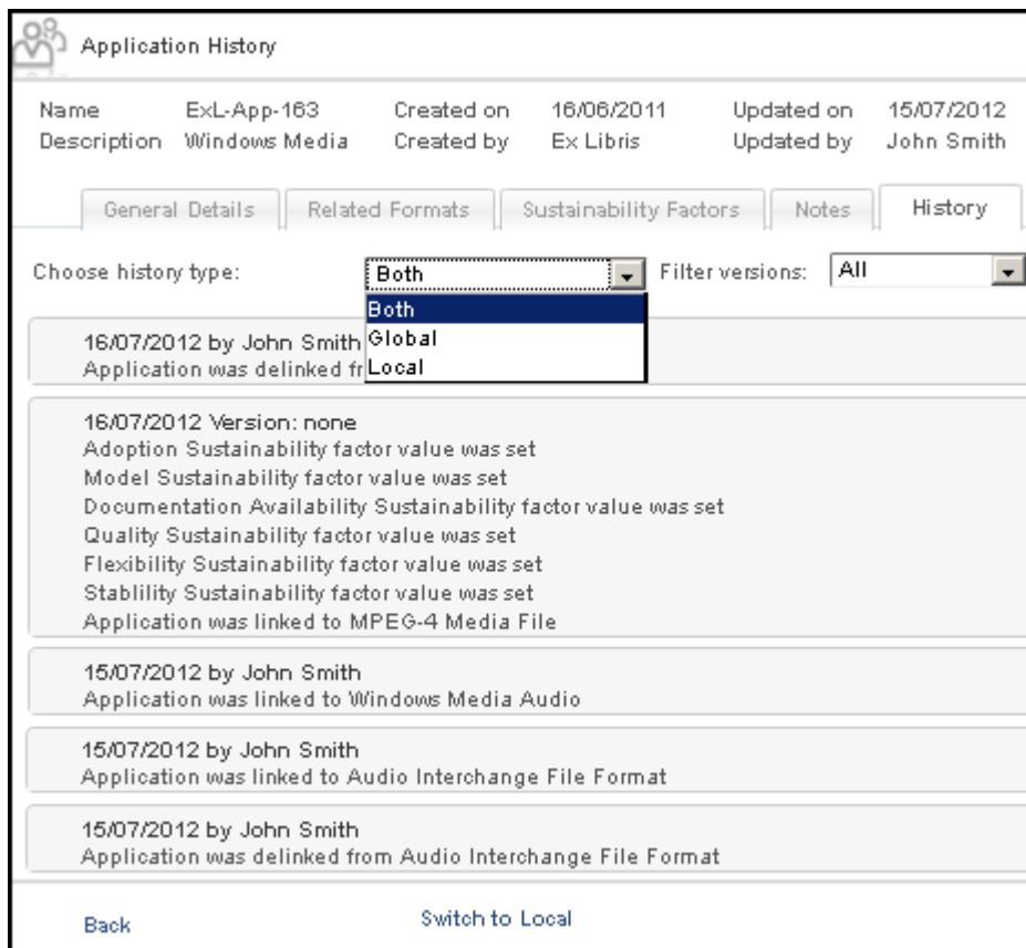
Figure 43: Application History
