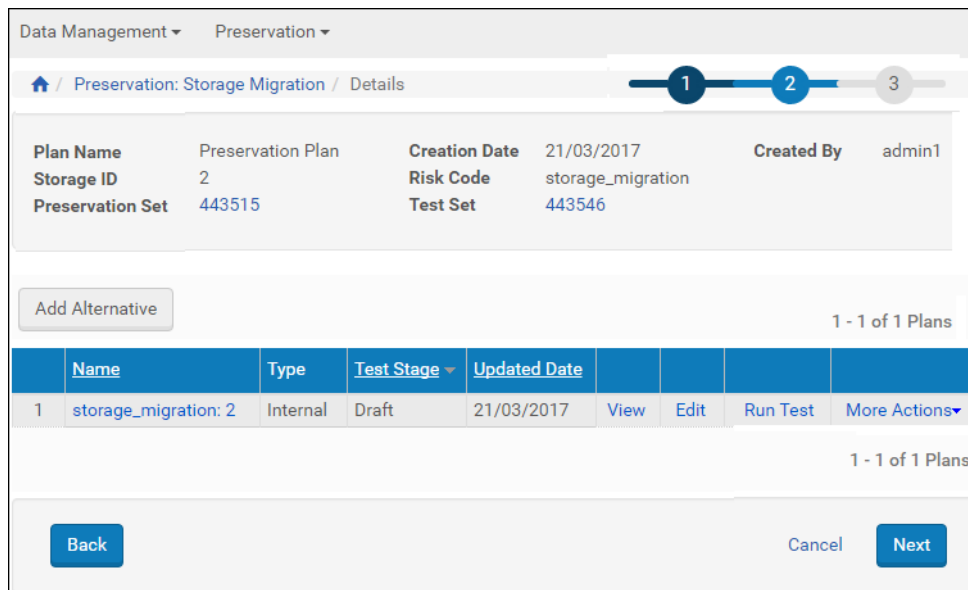
Figure 152: Add Alternatives
