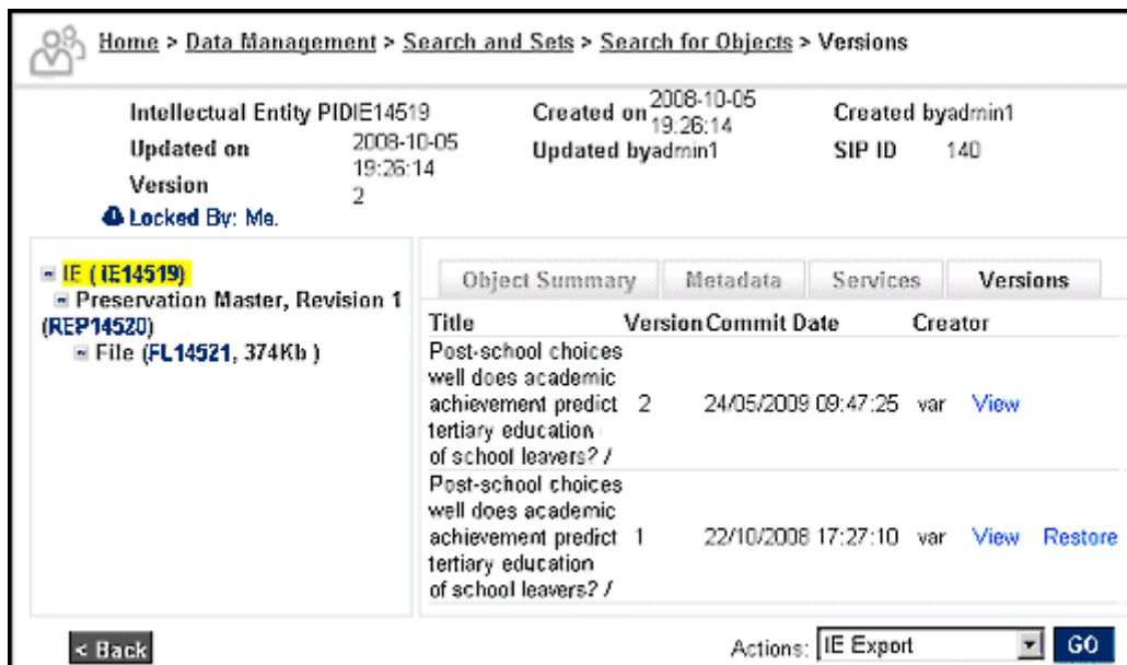
Figure 194: Version Tab of the Web Editor
