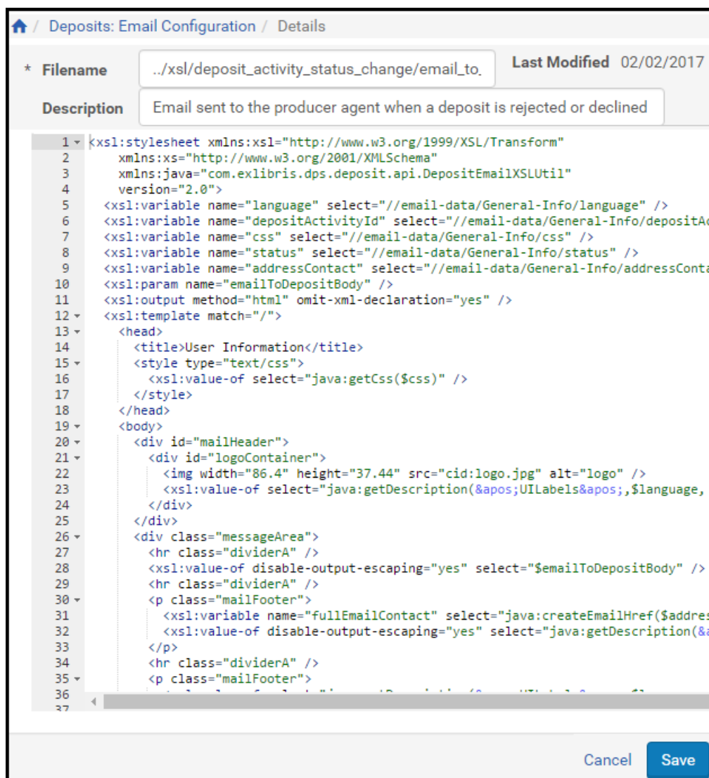
Figure 53: Editing a Configuration File
