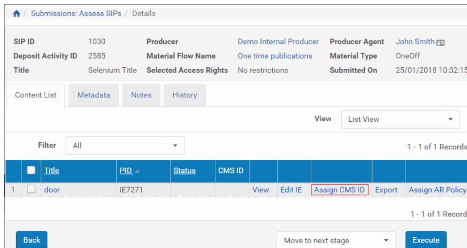
Figure 135: SIP Content List Page
