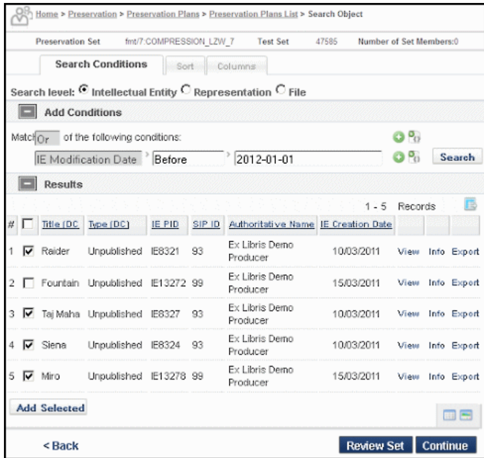
Figure 102: Search Object Page
