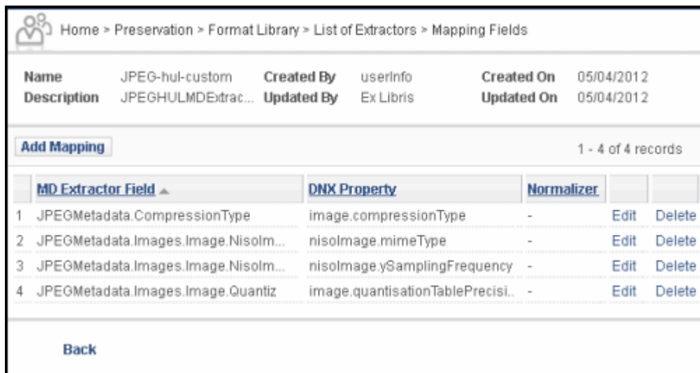
Figure 64: Editing a Custom Extractor
