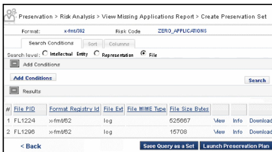
Figure 75: Post-query Search Object page
