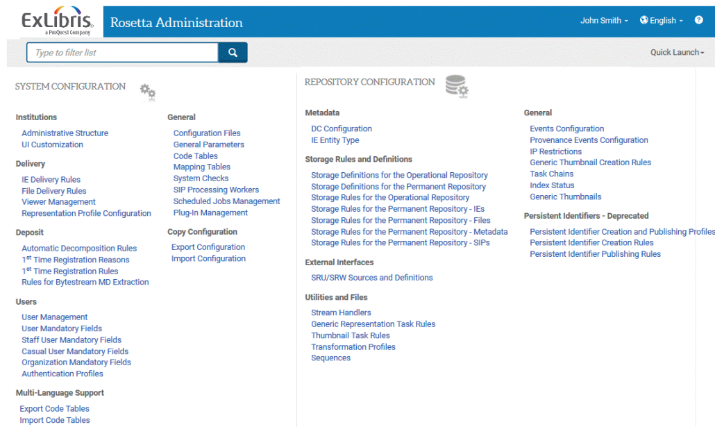
Figure 4: Administration/Consortium-wide Menu
