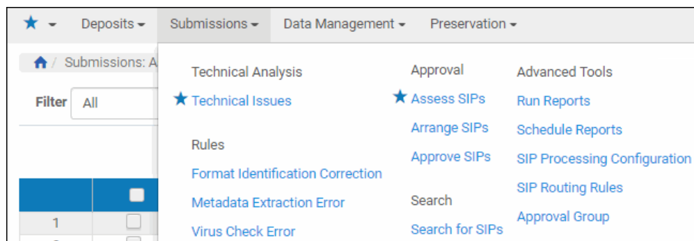
Figure 13: Submissions Menu
